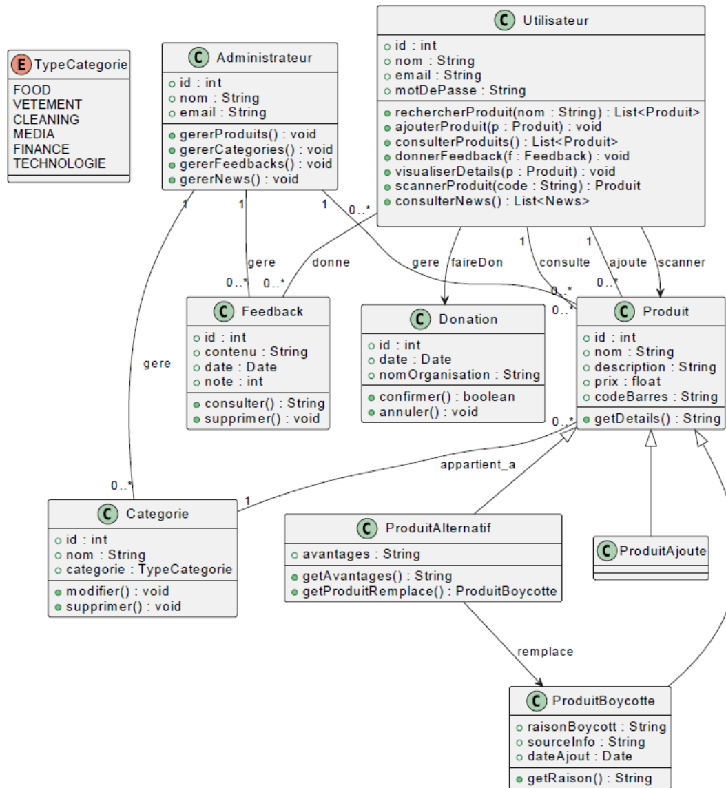
FIGURE 2.3 – Diagramme de classes
