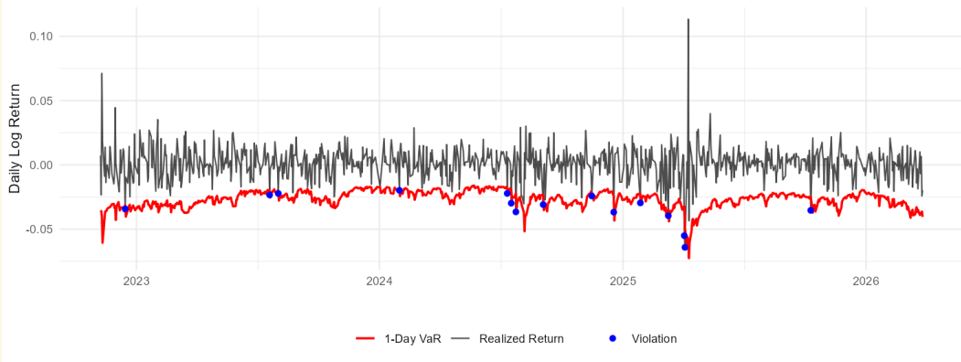
VaR Backtest: GARCHX with VIX Overlay
