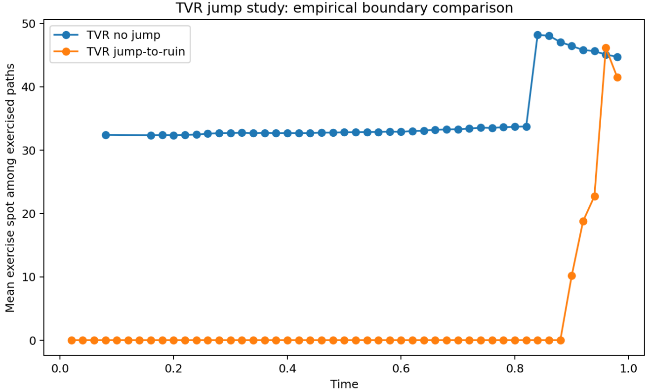
Figure 7: Jump-style boundary comparison: TVR.
