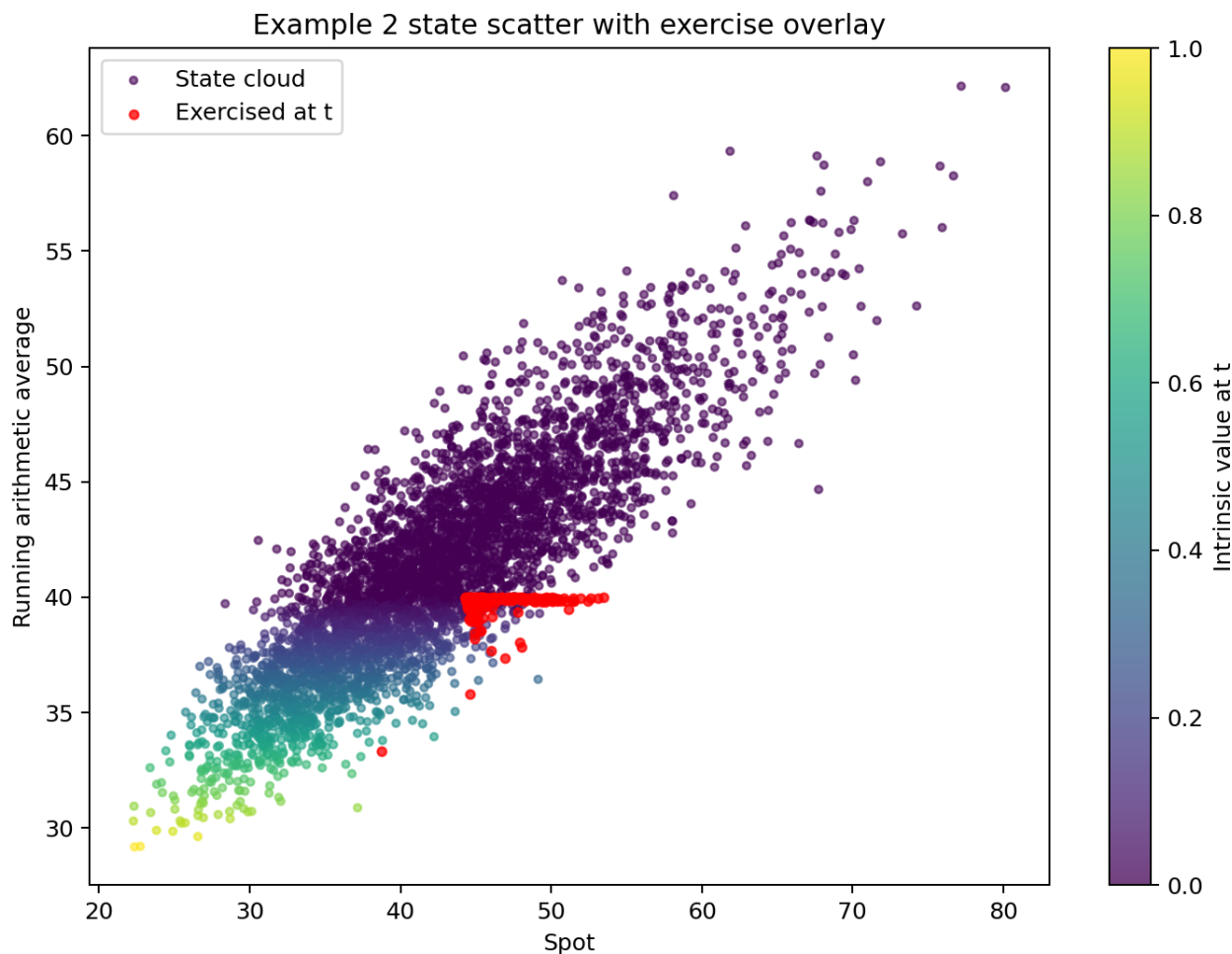
Figure 4: Asian-style state cloud with exercise overlay: Longstaff.
