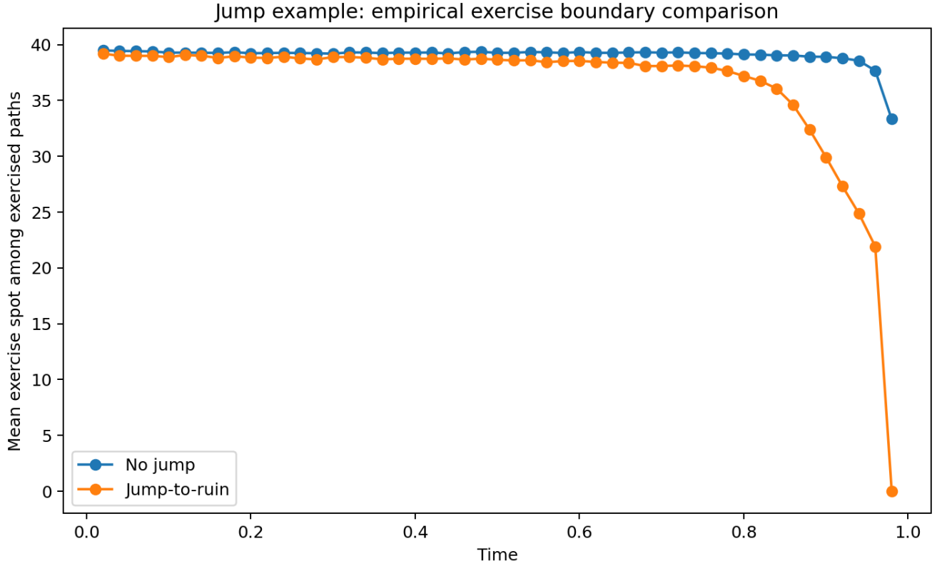
Figure 6: Jump-style boundary comparison: Longstaff.
