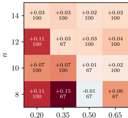
Watts-Strogatz
