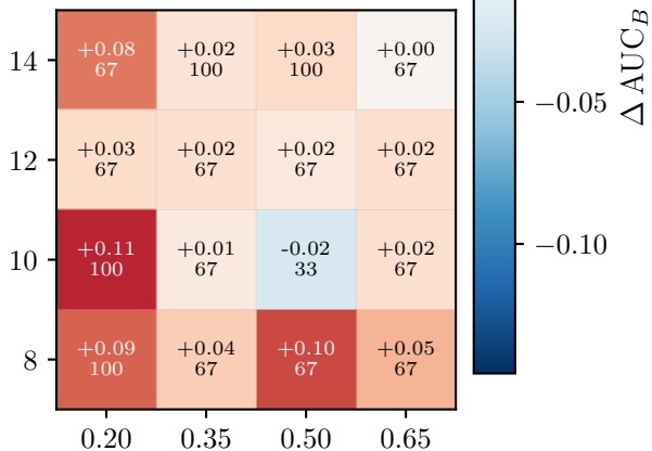
Barabasi-Albert
