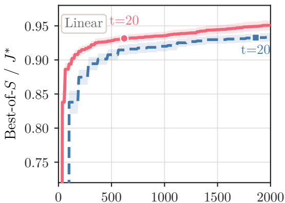
Best-of- S
