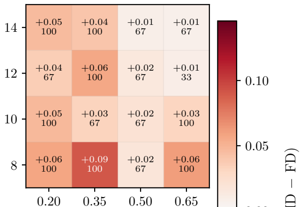
Barabasi-Albert
