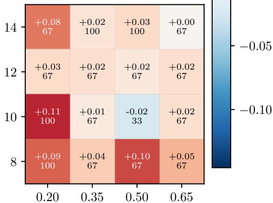
Barabasi-Albert
