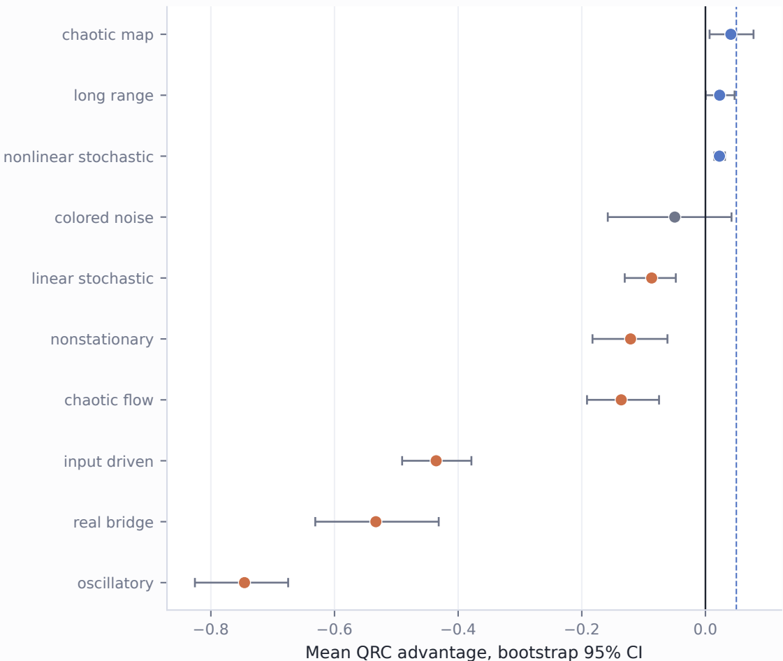
Family mean advantage intervals
