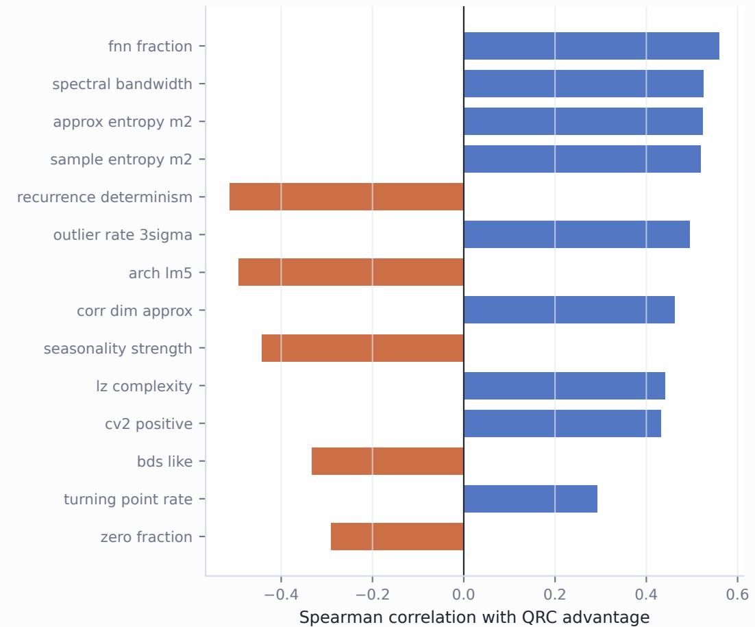
Extended descriptors most aligned with usefulness
