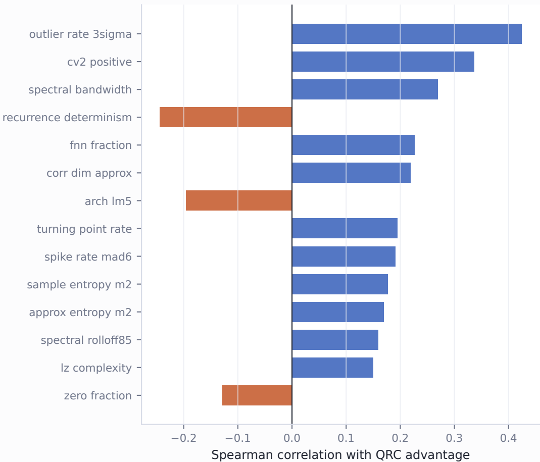
Extended descriptors most aligned with usefulness
