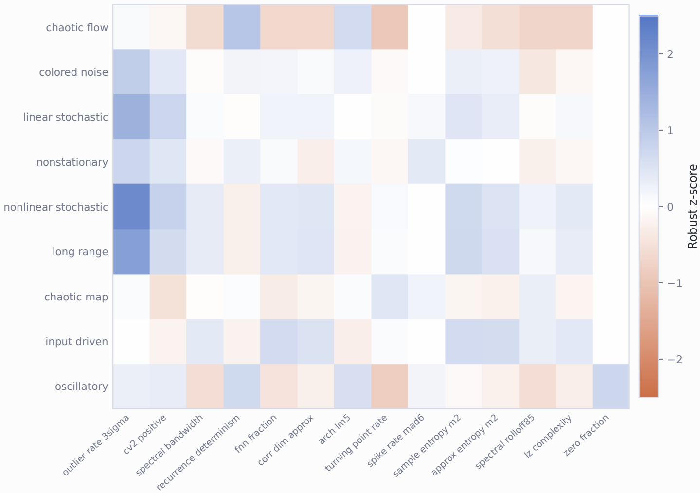
Family-average standardized feature structure
