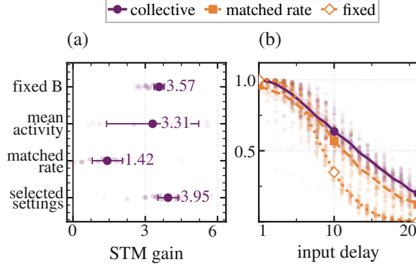
Figure 7: Targeted scalar controls preserve the local-collective memory contrast. (a) STM gain of collective over local relaxation under four separate comparisons: fixed assigned weight, matched mean activity, matched relaxation rate, and independently selected settings. Values above zero favor collective relaxation. (b) Memory from each previous input before and after the local relaxation rate is matched to the collective relaxation rate. The purple curve remains higher, so collective relaxation retains more input history even after that matching. Pale marks show individual reservoir pairs; large symbols, lines, bars, and bands show means and 95% intervals.
