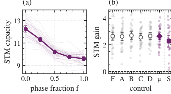
Figure 8: Accessible memory depends on the matched rank-one direction. (a) Prespecified N = 5 phase path. (b) Equal-phase-minus-control effects for five zero-overlap directions, their within-pair mean \mu , and the N = 6 sign-balanced replication S. Marks show pairs, means, and 95% t intervals (32 and 24 pairs).
