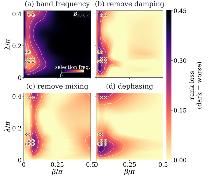
Fig. 3. Mechanism ablations destroy the operating band. (a) Selection frequency in the original reservoir: for each coordinate (\beta, \lambda) , the color shows how often it reaches top-quintile validation rank across the 80 task–seed replicates; gold circles mark the B_{20,0.7} band. (b)–(d) Validation-rank loss for three representative ablations named in the panels, with darker colors indicating larger deterioration. The strongest losses occur at the original band coordinates.
