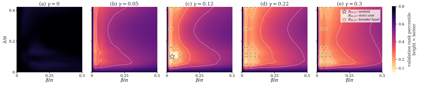
Fig. 4. Appendix damping-slice atlas for the same validation-ranked grid. Each panel fixes \gamma and maps validation rank over (\beta, \lambda) , with bright color indicating better rank. All marked points use the same consistency requirement q = 0.7 : filled circles show the strict B_{20,0.7} core, open circles show the broader B_{30,0.7} band, and the star marks the B_{20,0.7} medoid. The strict core sits at \gamma = 0.12 , while the broader same-consistency band extends into neighboring nonzero damping slices.
