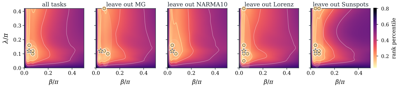
Fig. 1. Validation phase maps at the fixed \gamma = 0.12 slice. Bright regions are low validation percentile rank. Gold circles mark points that appear in the top-20% for at least 70% of the displayed task-seed replicates; the star is the medoid of the primary band. The same low-input, nonmaximal-coupling region persists under leave-one-task-out conditioning.
