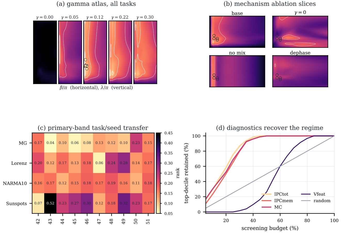
Fig. 2. QRC-only evidence for the operating-regime hypothesis. (a) Gamma-slice atlas: the useful region emerges only away from zero damping and away from maximal coupling. (b) Focused ablations at \gamma = 0.12 : outlines show the base B_{20,0.7} projection; \gamma = 0 , no-mix, and dephasing controls do not preserve it as a robust top region. (c) Task-seed transfer ranks for the primary band. (d) Intrinsic memory and processing-capacity diagnostics recover top validation-decile reservoirs more efficiently than random or diversity-only screening.
