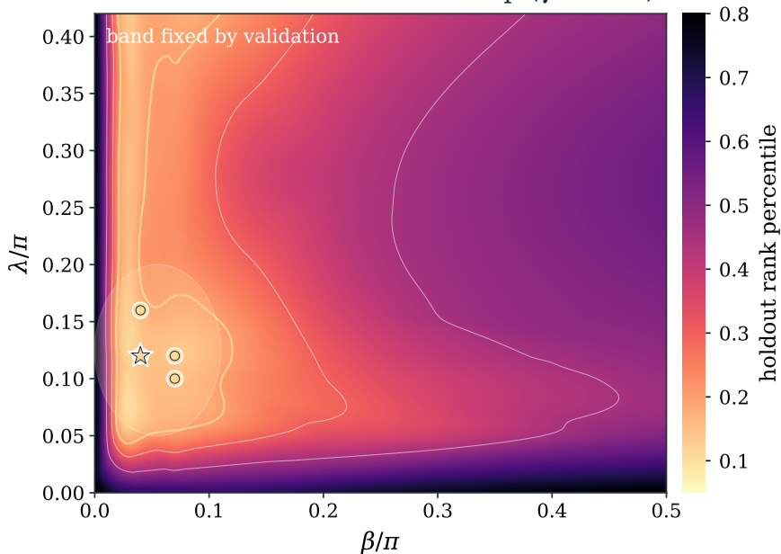
Candidate 1: holdout rank map ( \gamma = 0.12 )
