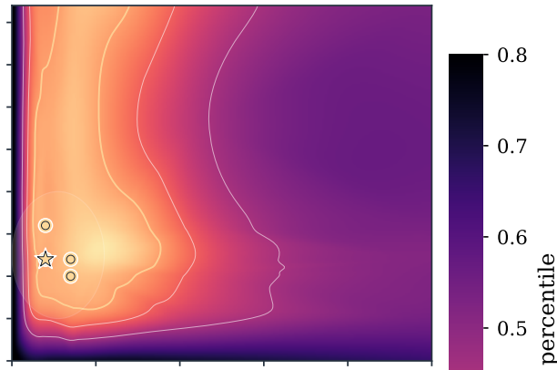
Sunspots
