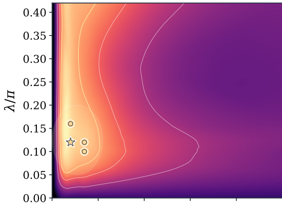
NARMA10
