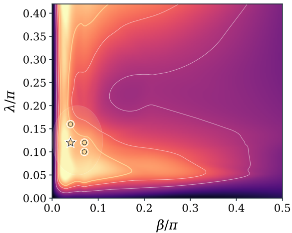
NARMA10
