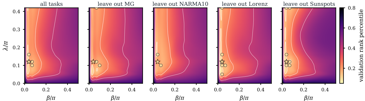
Phase maps transfer under leave-one-task-out conditioning ( \gamma = 0.12 )
