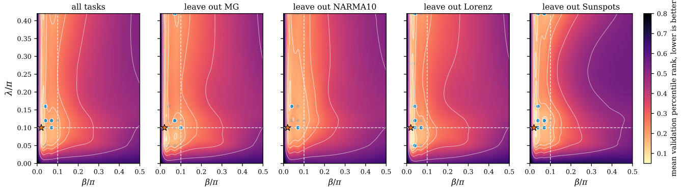
Memory-defined operating regime in a dissipative gate-model QRC ( \gamma = 0.12 slice)
