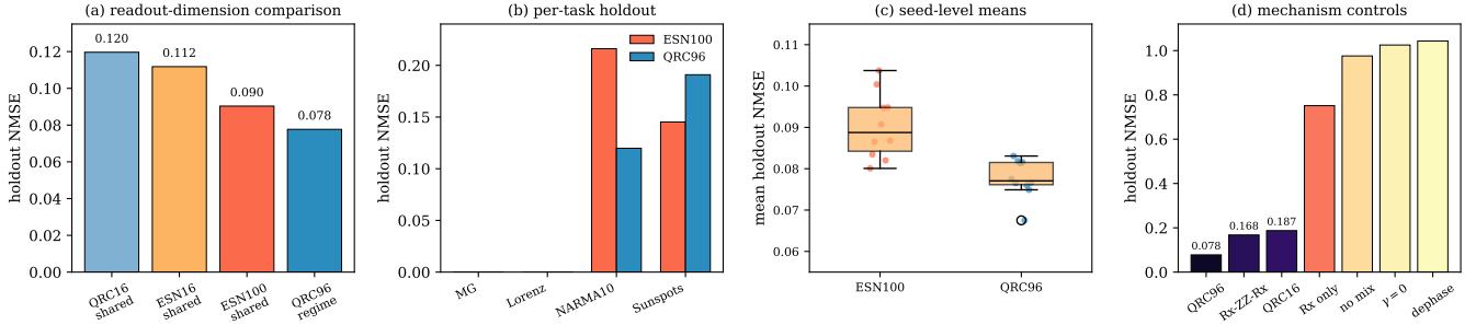
Fig. 2. Performance and mechanism controls. (a) QRC16 loses to both ESN baselines, while the memory-regime-targeted QRC96 readout improves the aggregate ESN100 comparison at matched readout dimension. (b) The QRC96 gain is mainly carried by NARMA10; Mackey–Glass and Lorenz are near floor, and Sunspots favors ESN100. (c) Seed-level task means are lower for QRC96 than for ESN100. (d) Removing the memory-preserving mechanism collapses performance: richer readout access helps only after recurrent mixing and nonzero damping establish usable memory.
