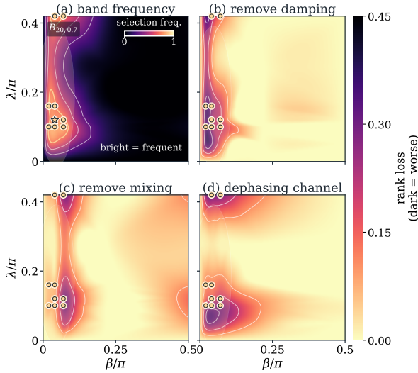
Fig. 3. Why the operating band is meaningful. (a) Bright coordinates are frequently selected by validation. (b–d) Removing damping, removing mixing, or replacing amplitude damping by dephasing concentrates rank loss around the same gold band, showing that the useful region depends on these mechanisms.
