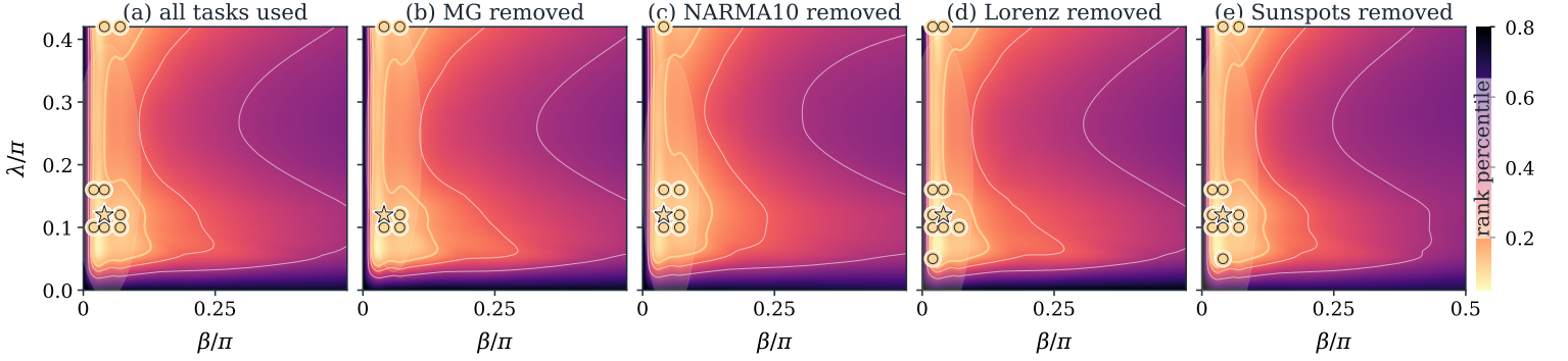
Fig. 1. Validation phase maps at \gamma = 0.12 , the first damping slice where the strict validation-defined band is populated. The full \gamma scan is shown in Fig. 2; this slice is used only for a readable 2D transfer view. The first panel uses all four tasks. Each following panel recomputes the map after removing one task from the validation aggregate. Gold circles mark coordinates that repeatedly fall in the top validation quintile; the star marks the primary-band medoid projected onto this slice.
