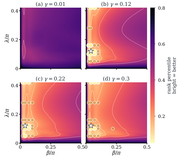
Fig. 2. Damping-slice check for the same validation-ranked grid. Bright color indicates better validation rank. The near-zero damping slice at \gamma = 0.01 provides a contrast, while the operating band appears across stronger nonzero damping slices.
