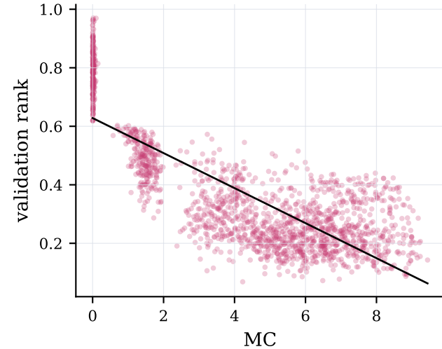
(a) memory capacity
