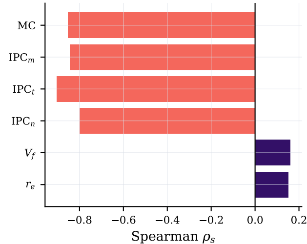
(c) diagnostic rank correlation
