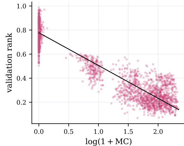
(b) log memory
