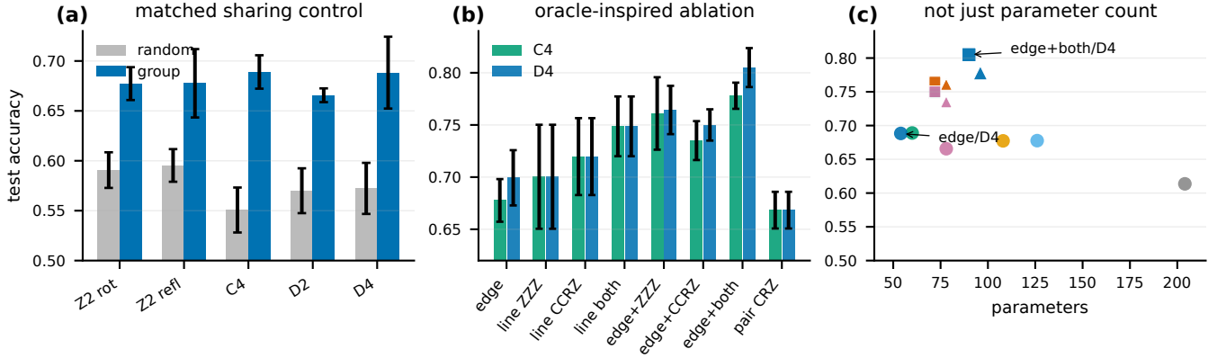
Fig. 3. Controls and ablations. (a) Parameter-matched random sharing underperforms group-orbit sharing, so the benefit is not only fewer parameters. (b) Oracle-inspired ablations at 600 training examples show that the strongest model combines edge interactions with both winning-line channels. (c) Accuracy is not explained by parameter count alone; task-aligned equivariant geometry is the relevant change.
