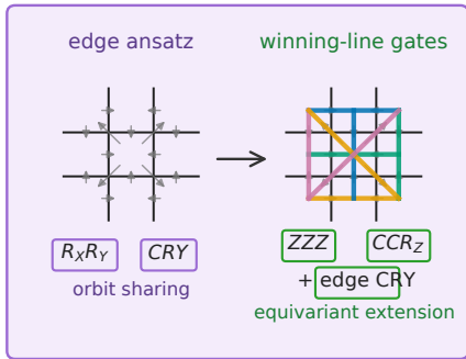
Equivariant gateset
