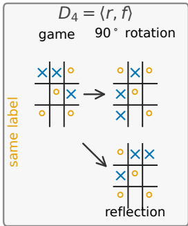
Symmetry
