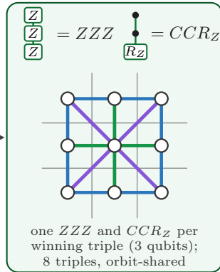
Our contribution
