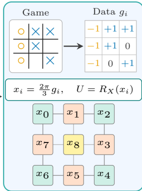
Shared encoding
