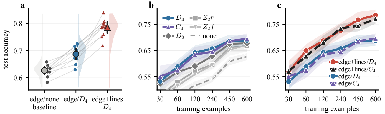
Fig. 2. Main results. (a) At 600 examples, no sharing is below the Meyer-style edge/ D_4 model, and our edge+lines/ D_4 model is higher still. (b) C_4 closely follows D_4 across train sizes. (c) Edge+lines gives the largest gain while preserving equivariance. Error bars are 95% confidence intervals over seeds.
