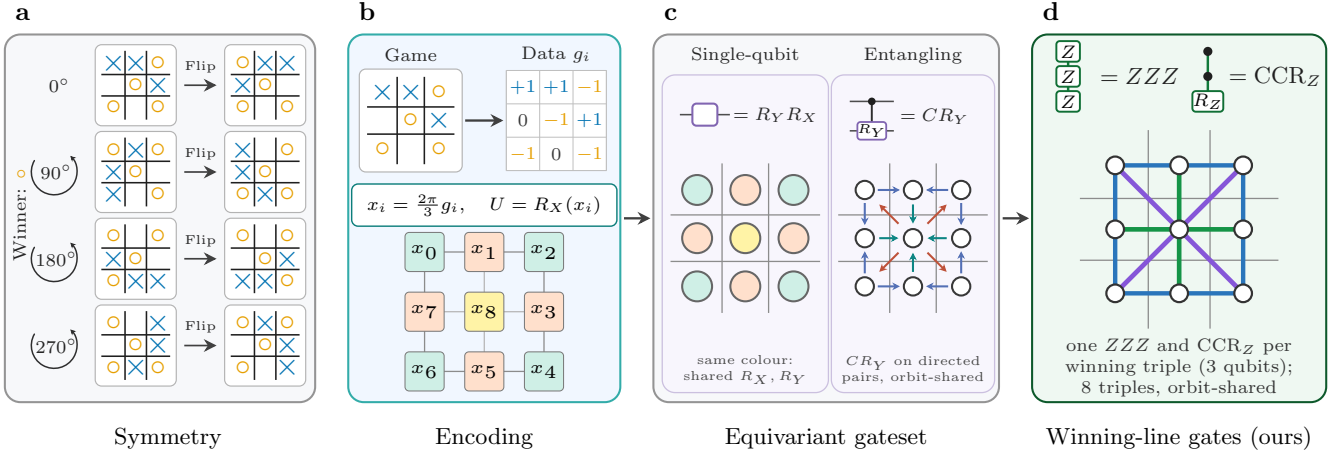
Fig. 1. From task symmetry to a task-aligned equivariant circuit. (a) Tic-Tac-Toe labels are invariant under the D_4 rotations and reflections of the board. (b) Board entries g_i \in \{-1, 0, +1\} are encoded as R_X(x_i) rotations with x_i = \frac{2\pi}{3}g_i ; the chosen indexing exposes the corner, side, and center orbits. (c) The Meyer et al. [9] edge ansatz uses orbit-shared R_Y R_X rotations and directed C R_Y entanglers on neighbouring and center-connected fields. (d) Our extension adds orbit-shared ZZZ and symmetric CCR_Z gates on the eight winning triples, directly matching the label-relevant motifs while preserving equivariance. Panel layout adapted from Meyer et al. [9].
