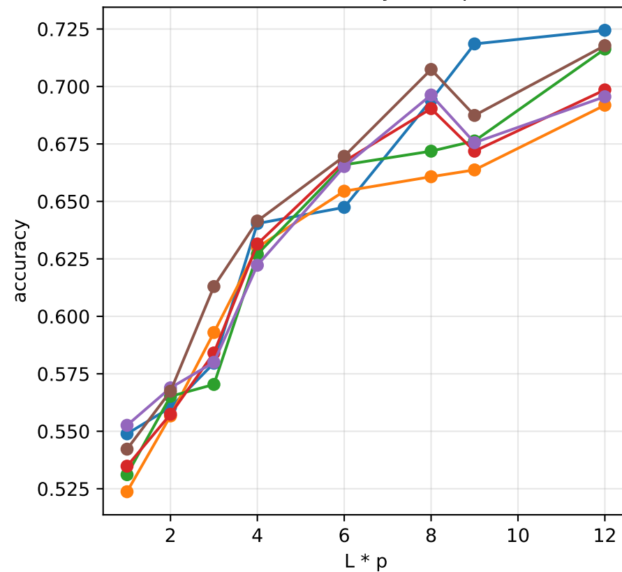
Train accuracy vs depth
