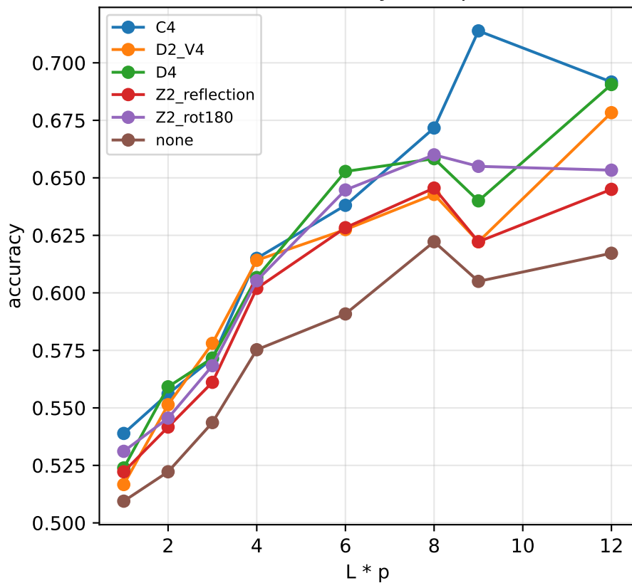
Test accuracy vs depth
