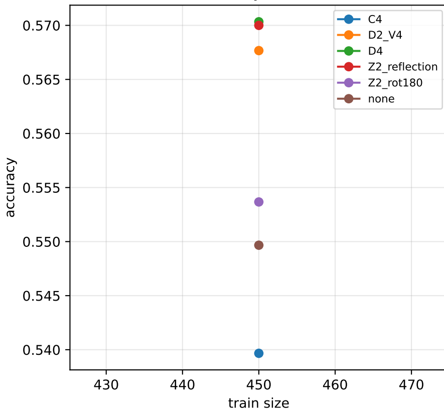
Test accuracy vs train size
