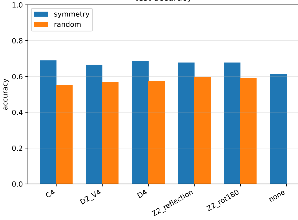
test accuracy
