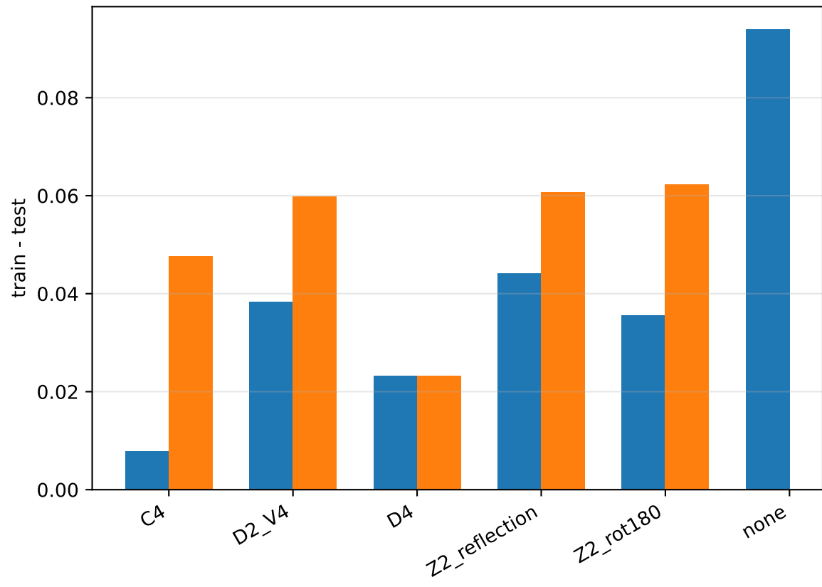
generalization gap
