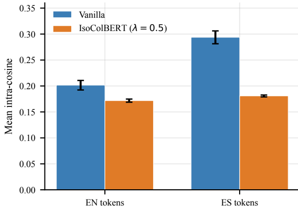
Intra-cosine (lower = more isotropic)
