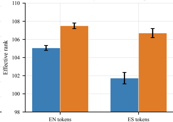
Effective rank (higher = more isotropic)
