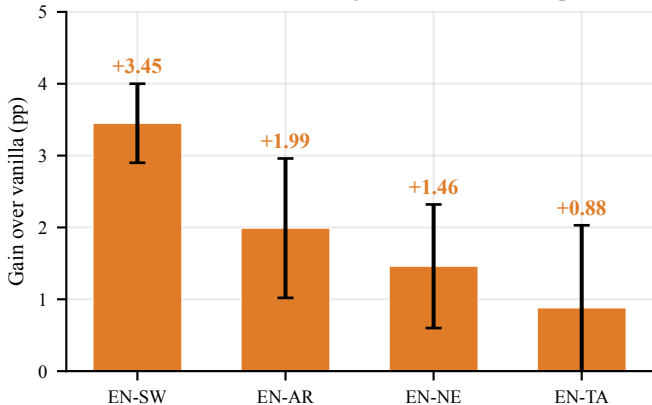
IsoColBERT ( \lambda = 0.5 ) gain on low-resource pairs
