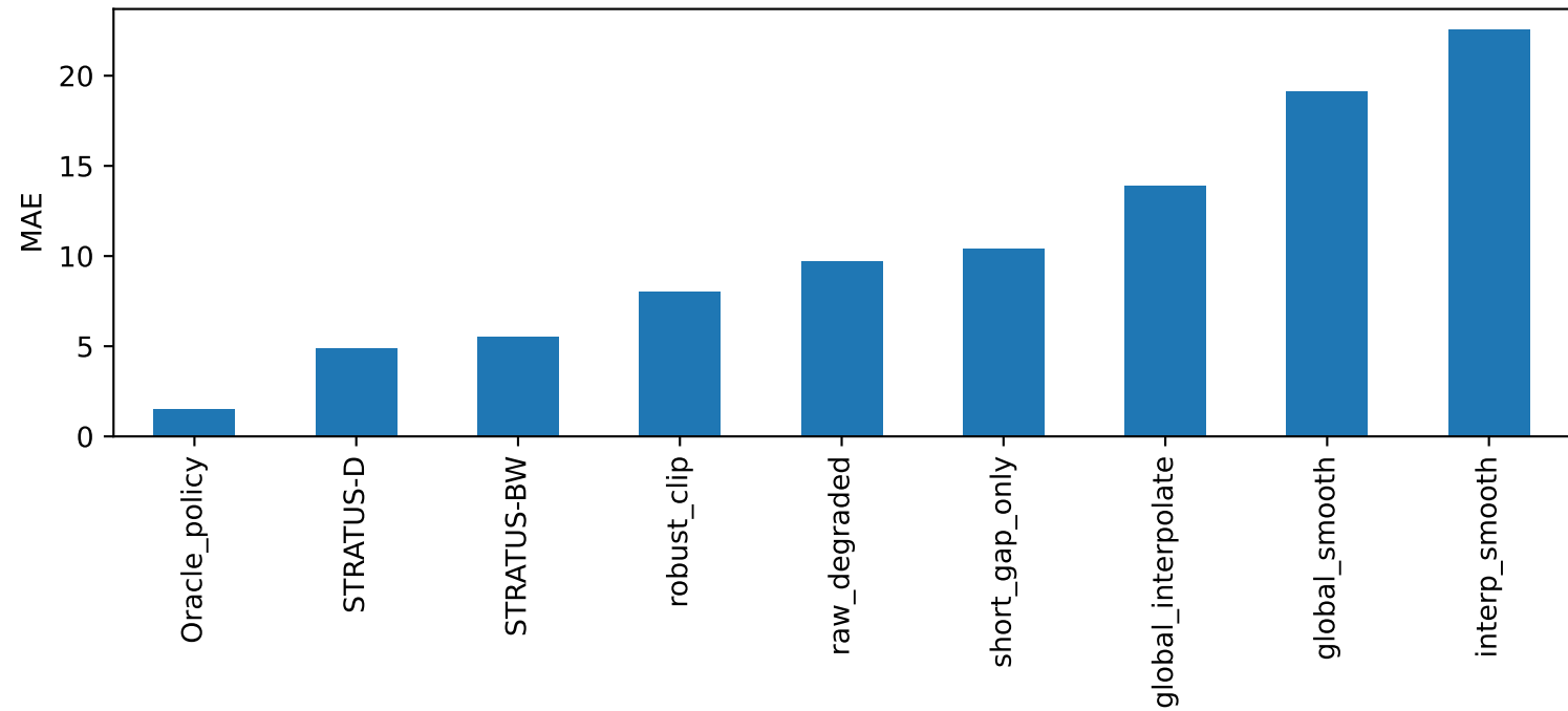
Dataset-macro reconstruction error by method
