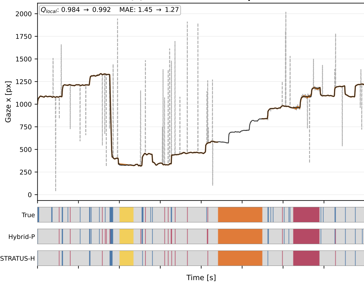
(a) ETDD70: mixed corruption
