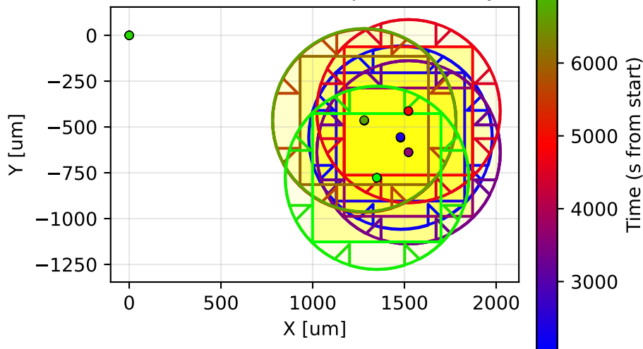
Stimulus Presentation Map (colored by time)
