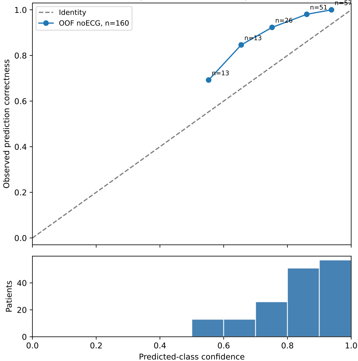
Supplement: predicted-class confidence 10 equal-width bins; descriptive
