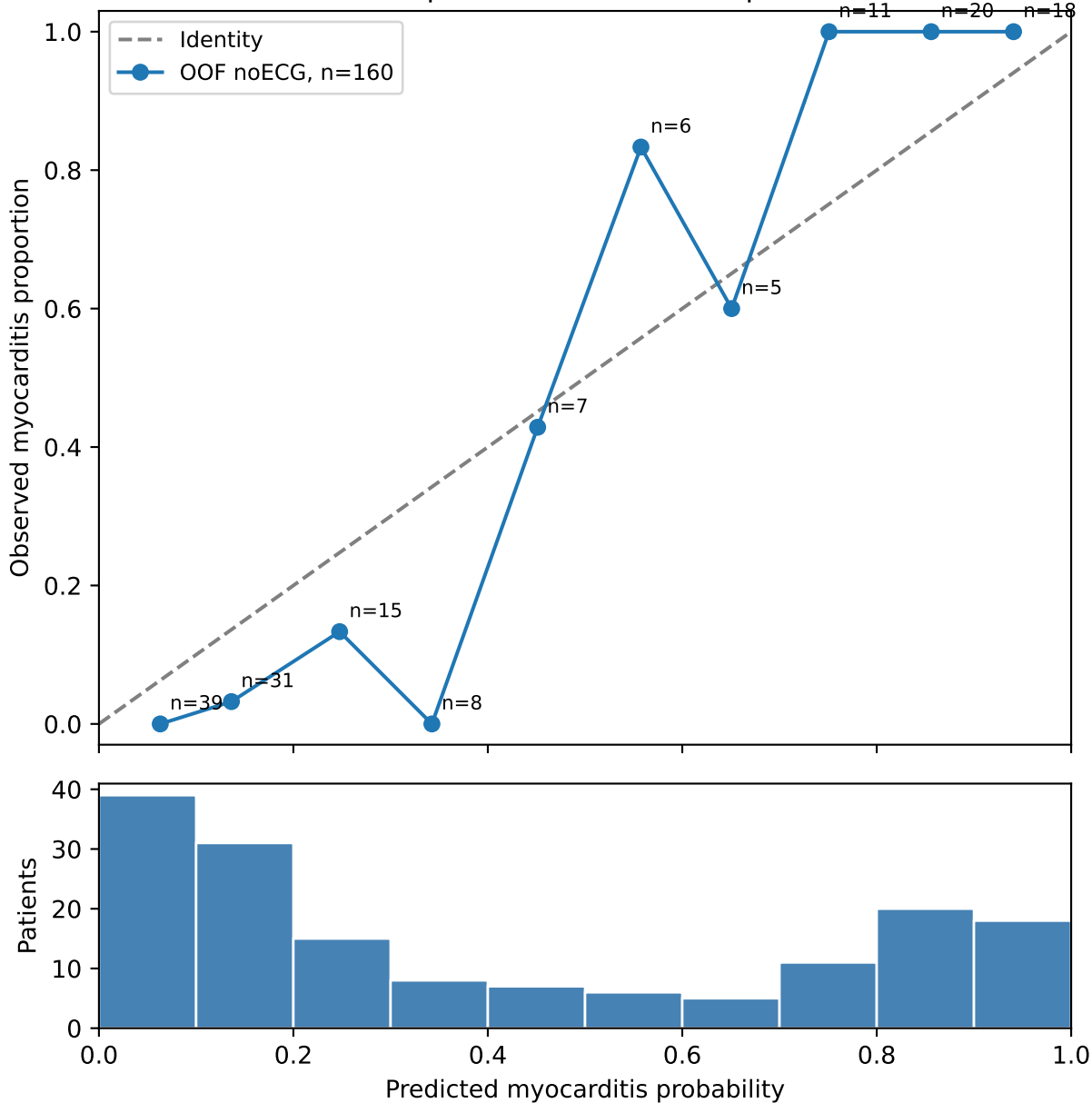
Primary: myocarditis probability 10 equal-width bins; descriptive
