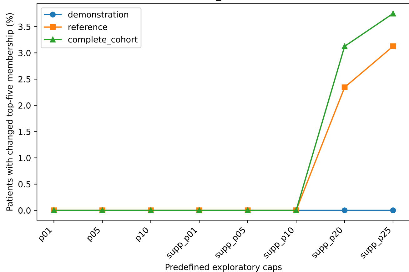
low_score
