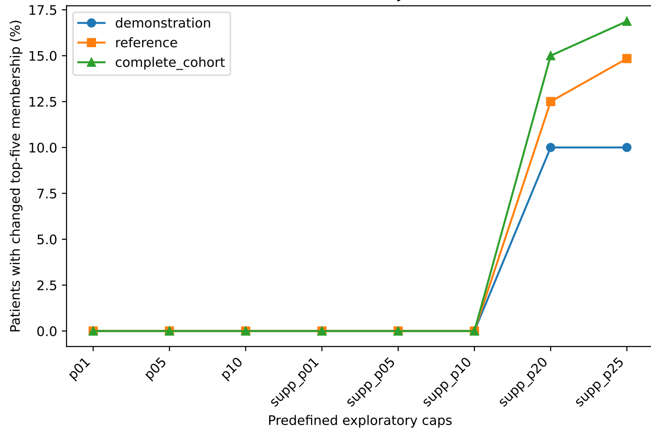
uncertainty
