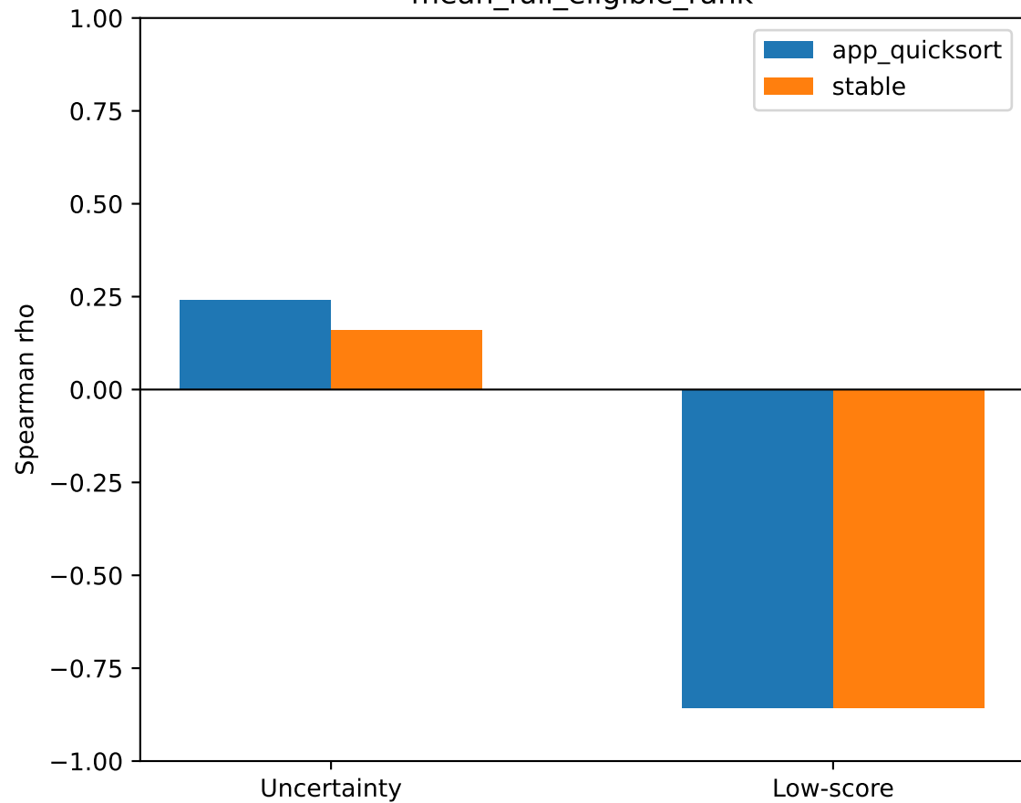
mean_full_eligible_rank
