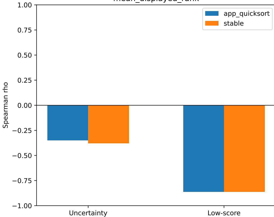
mean_displayed_rank
