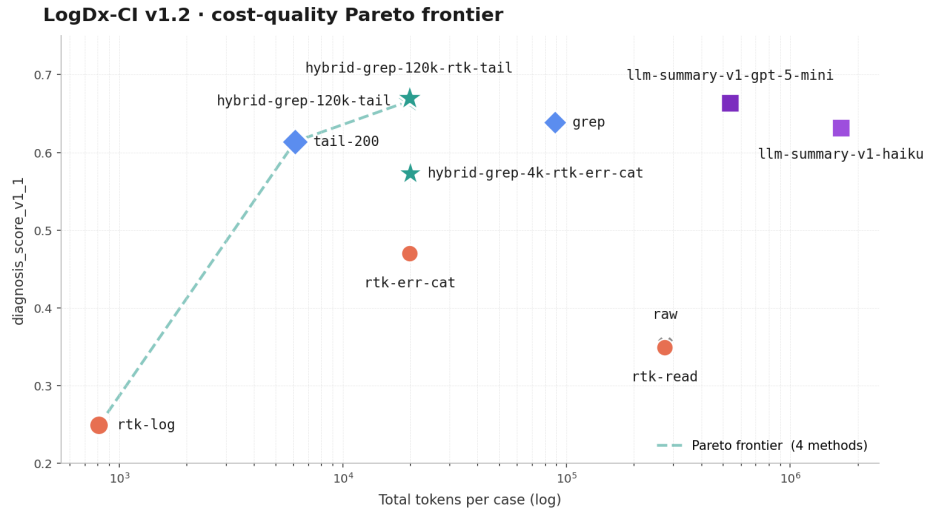
Figure 1: Cost-quality Pareto frontier across 11 log-reduction tools. Case-count-weighted macro diagnosis_score_v1_1 across the 35-case corpus \times 3 single-shot LLM debugger families. Green dashed line traces the 4-method frontier (rtk-log \rightarrow tail-200 \rightarrow hybrid-grep-120k-tail \rightarrow hybrid-grep-120k-rtk-tail); all other methods are dominated. The top two hybrids reach 0.670 / 0.666 at \sim 20k tokens per case — 4.5 \times fewer tokens than grep at same-ballpark quality . See §4.1–§4.4.
