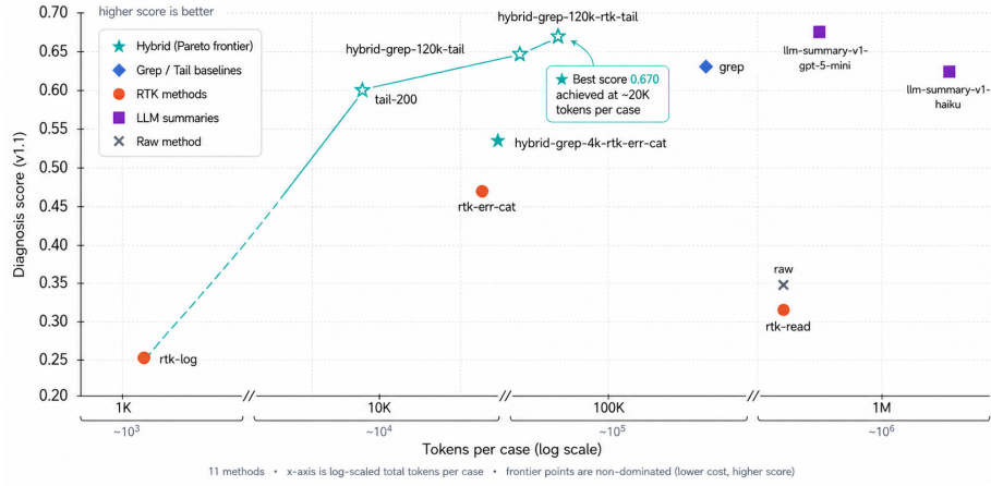
Figure 1: Cost-quality Pareto frontier across 11 log-reduction tools. Case-count-weighted macro diagnosis_score_v1_1 across the 35-case corpus \times 3 single-shot LLM debugger families. Green dashed line traces the 4-method frontier (rtk-log \rightarrow tail-200 \rightarrow hybrid-grep-120k-tail \rightarrow hybrid-grep-120k-rtk-tail); all other methods are dominated. The top two hybrids reach 0.670 / 0.666 at ~20k tokens per case — 4.5 \times fewer tokens than grep at same-ballpark quality . See §4.1–§4.4.
