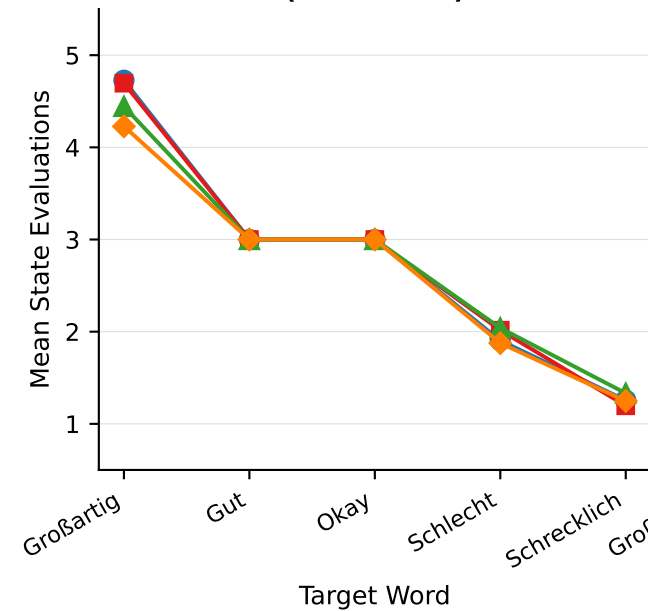
Behavioral (LLM choice)
