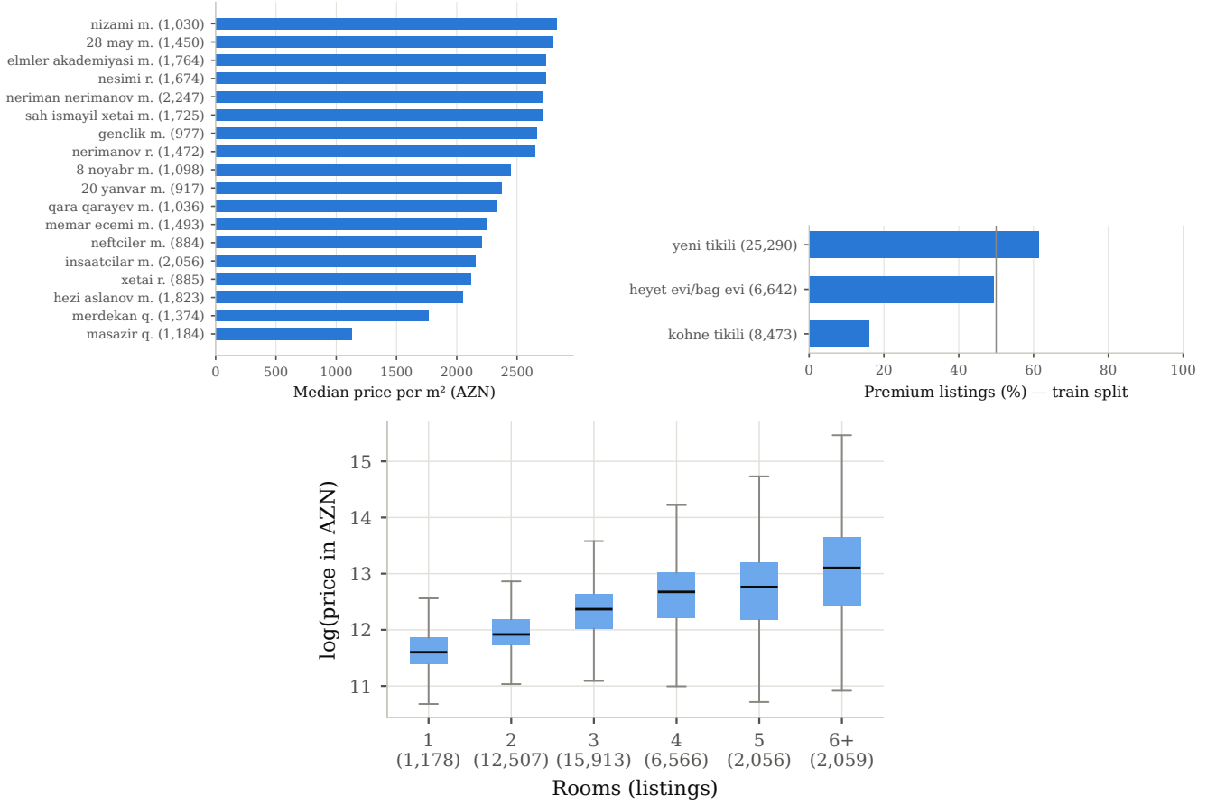
Figure 7. Location effect (median price per m 2 by district, training listings in brackets), premium share by category, and log price by room count (training split).
