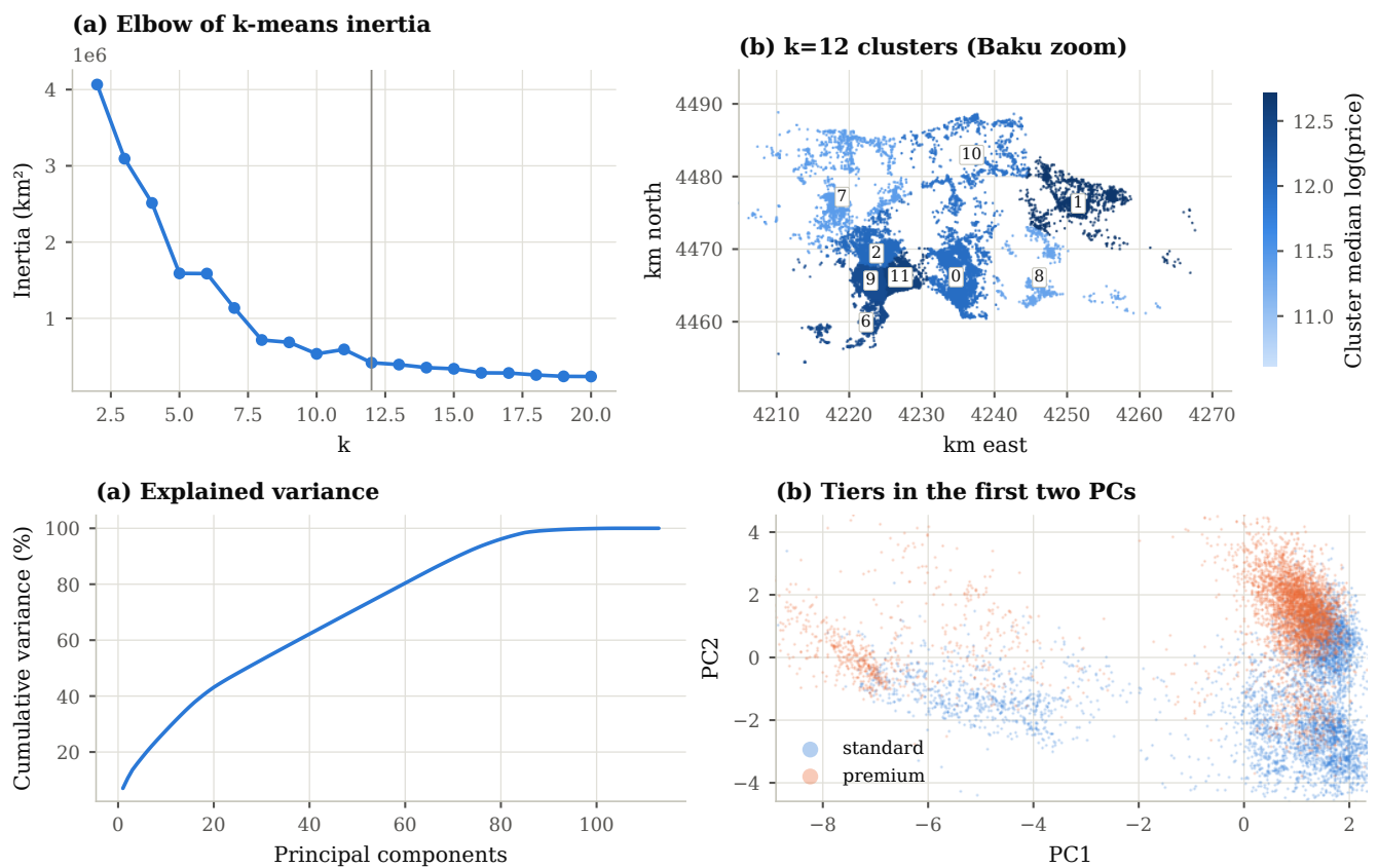
Figure 12. Bonus: k-means elbow and geographic clusters coloured by median log price; PCA explained variance and the two tiers in the first two components.
