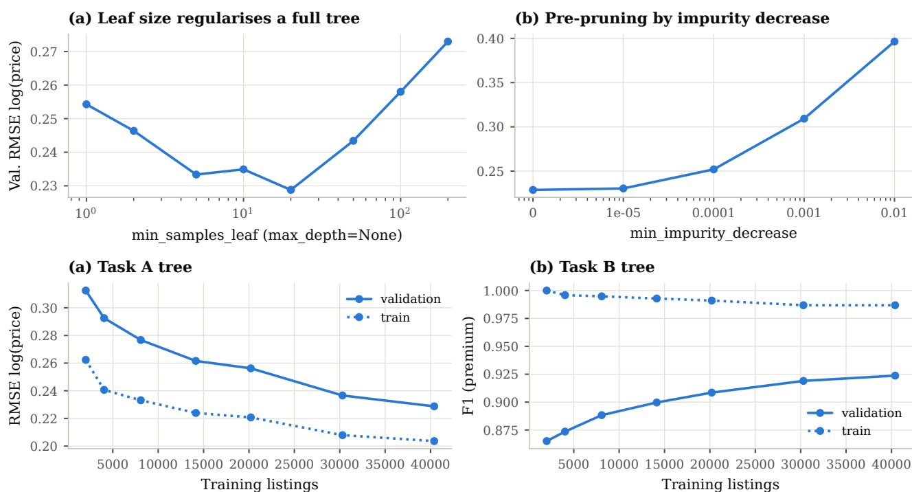
Figure 9. Top: validation RMSE vs. min_samples_leaf for a fully grown tree, and vs. min_impurity_decrease at the selected depth. Bottom: learning curves of the selected trees.
