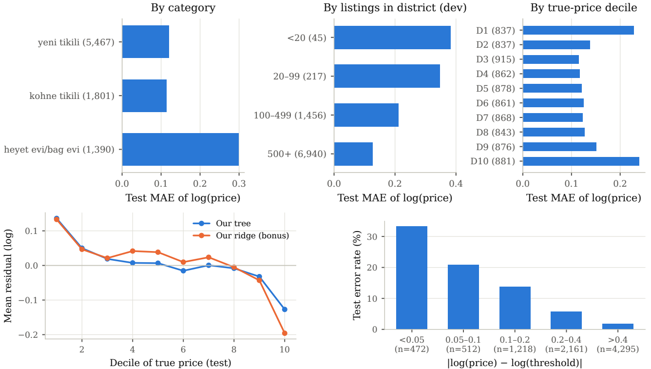
Figure 5. Error analysis on the test split. Top: Task A MAE of \log(\text{price}) by category, by number of training listings in the district, and by true-price decile (row counts in brackets). Bottom left: mean residual per price decile; the tree pulls the extremes towards the mean. Bottom right: Task B error rate vs. distance from the threshold. A map of the residuals is in the appendix (Fig. 8).
