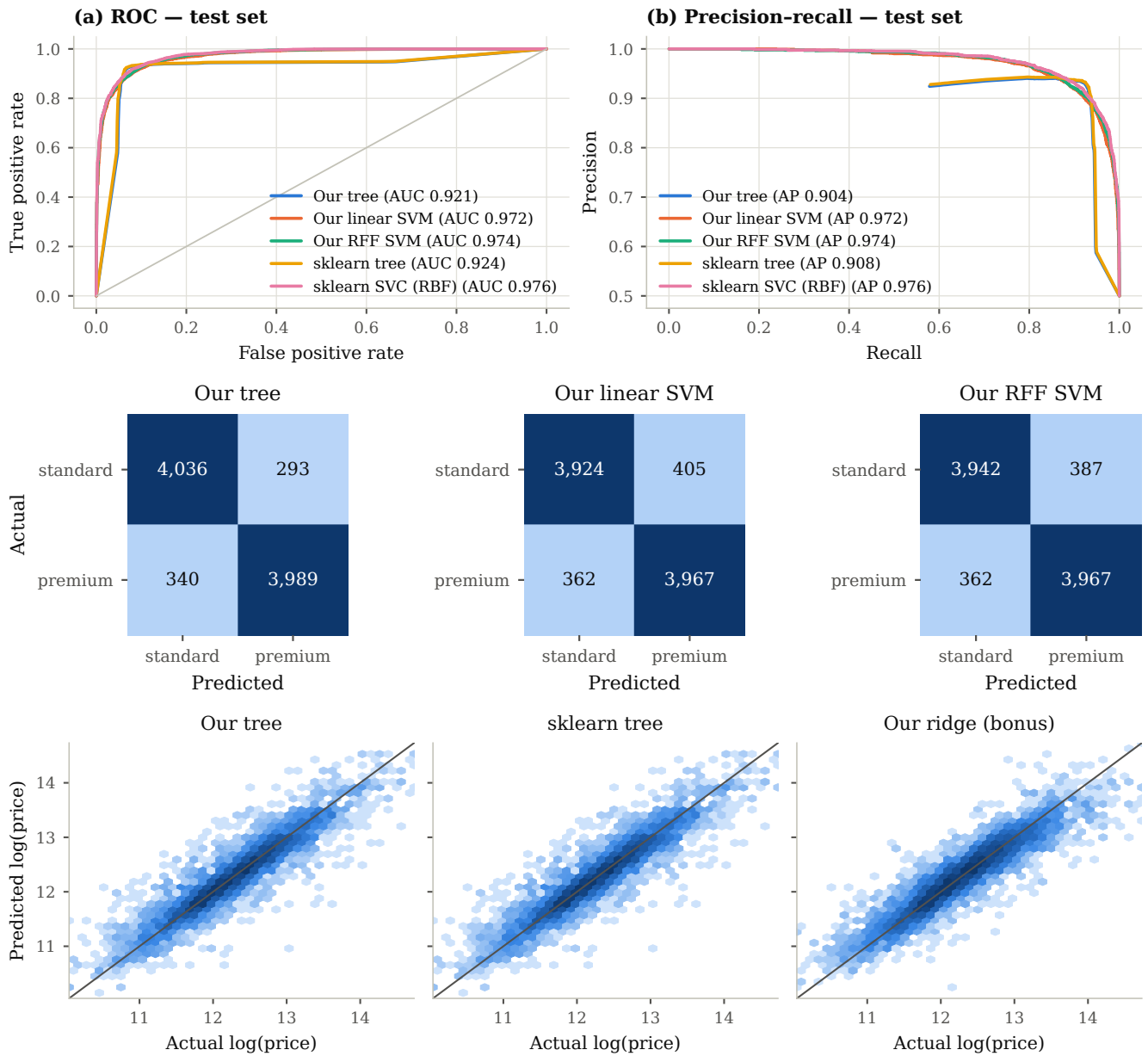
Figure 10. Test-set ROC and precision–recall curves, confusion matrices, and predicted vs. actual log price.
