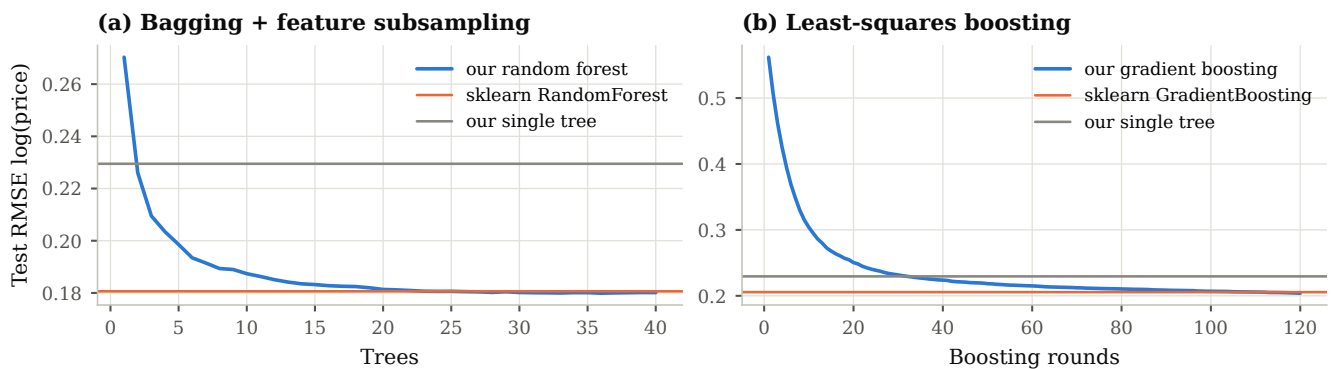
Figure 11. Bonus: test RMSE as learners are added to our random forest (a) and our gradient boosting (b), with scikit-learn's final value and our single tree as references.
