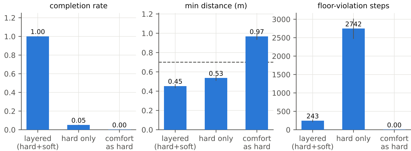
E3.3 — soft/hard layering on S3 bottleneck (20 seeds): removing the soft tier costs BOTH liveness and safety; hardening comfort clogs the funnel
