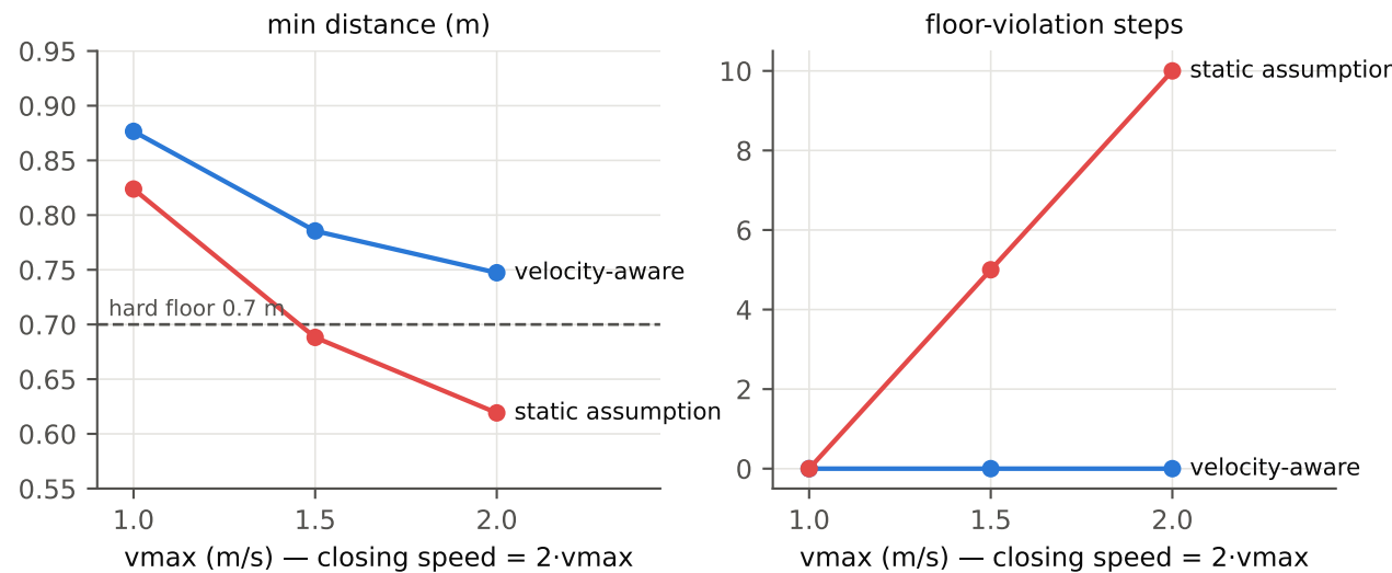
E3.5 — velocity-aware prediction on S2 head-on (20 seeds): the static assumption halves the perceived closing rate and dips deeper as speed rises
