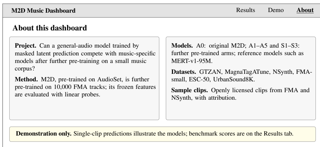
Figure 4.7: Wireframe of the About page (FR-18). Two text panels describe the project question and method on the left, and the models, datasets and sample-clip licenses on the right. A highlighted box at the bottom states that single-clip predictions are a demonstration and that the benchmark scores are those on the Results tab.
