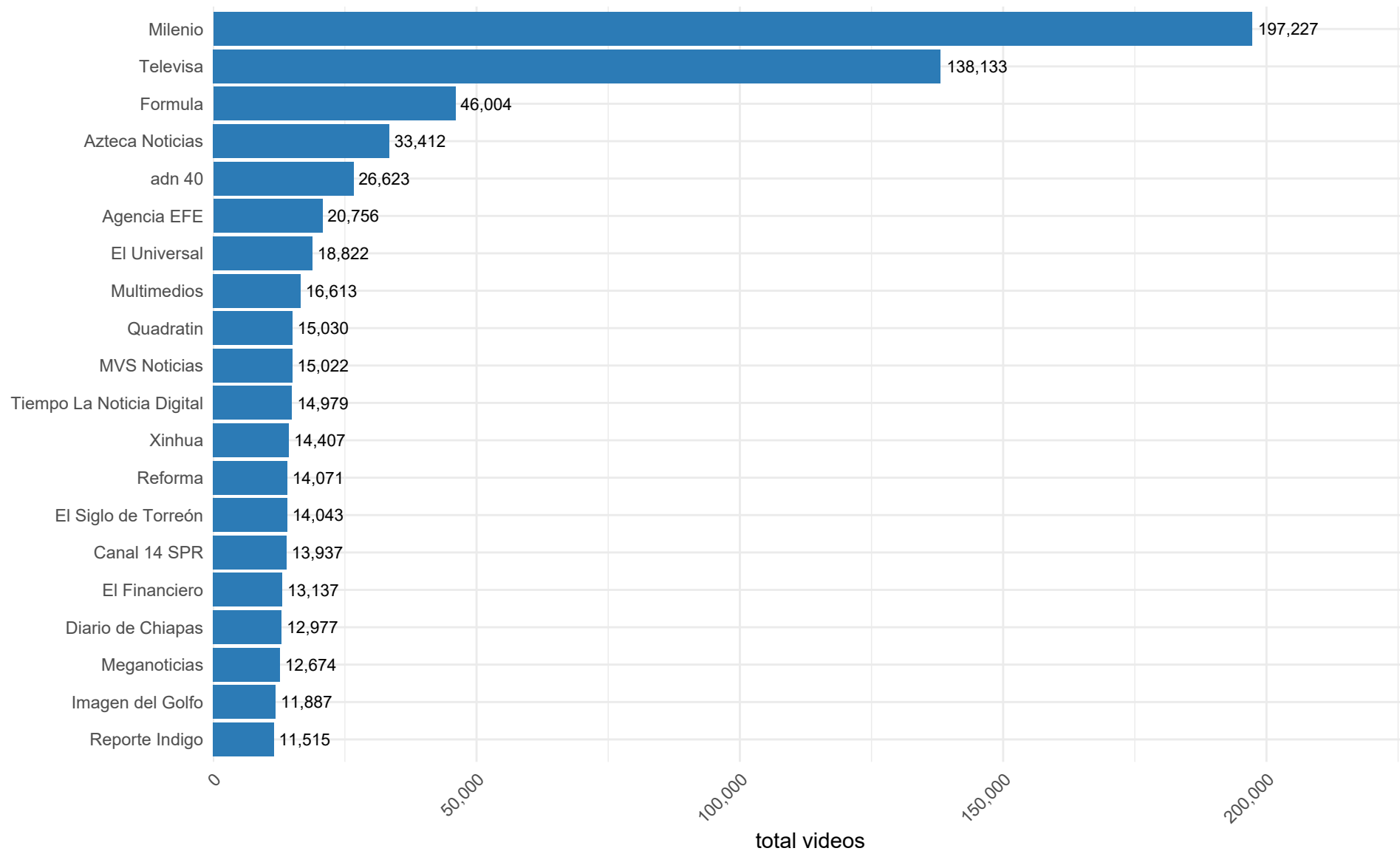
Top 20 channels by total videos published (2018-2024)
