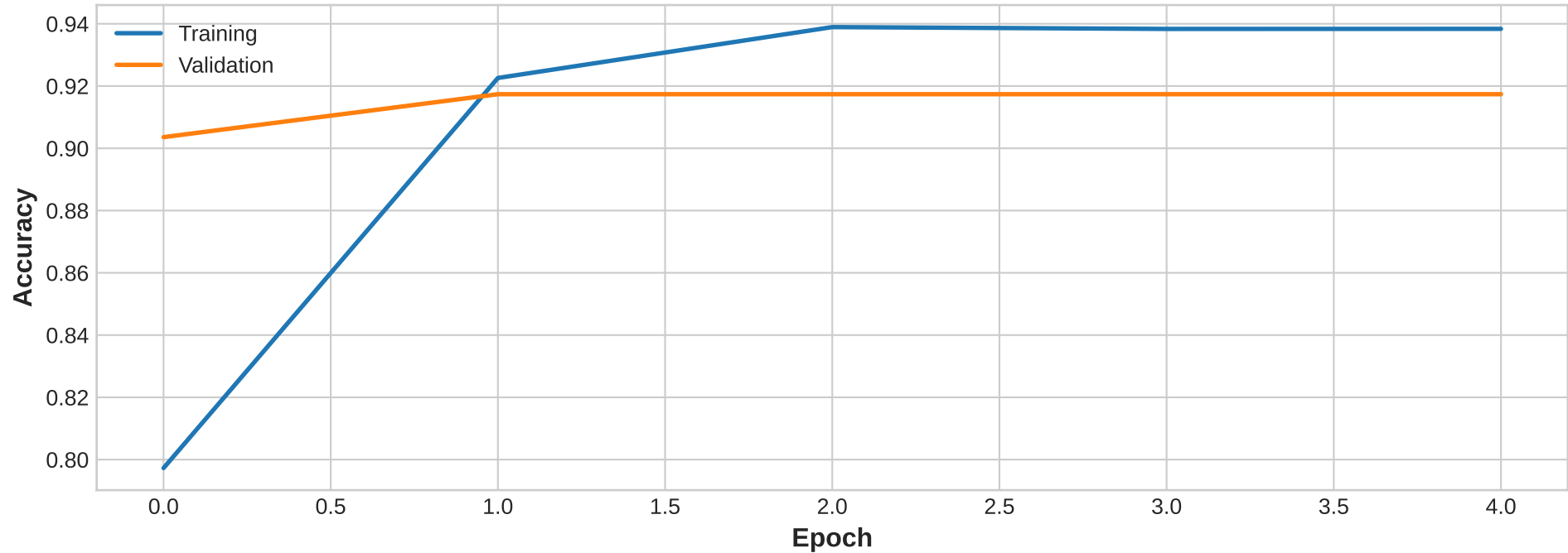
Categorical accuracy
