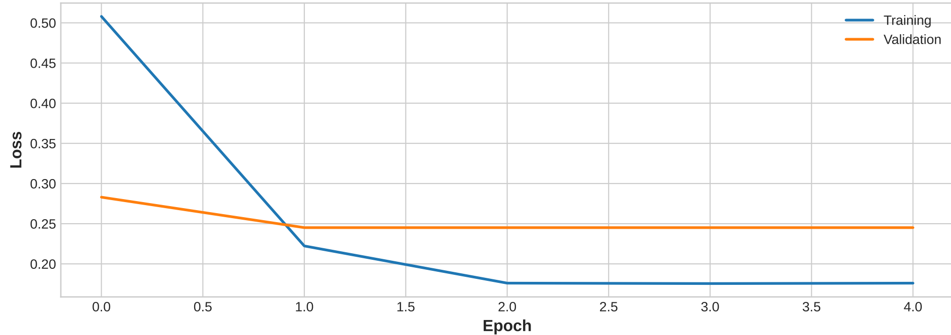
Loss
