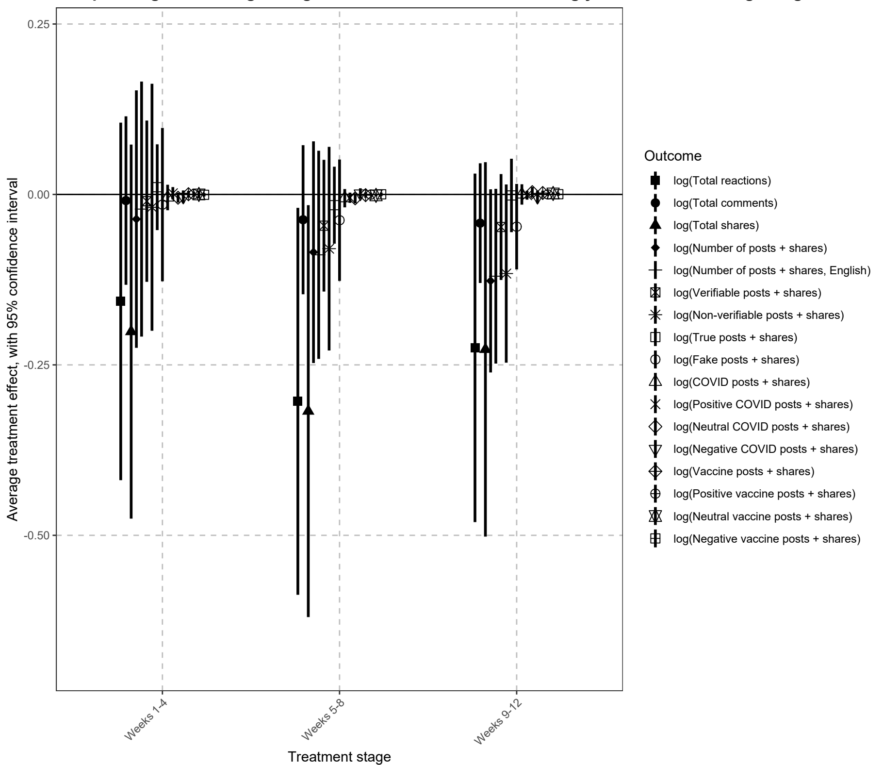
Sample-weighted average marginal effect of an additional strongly-followed SMI being assigned to treatment
