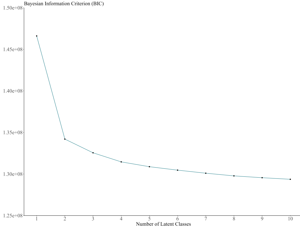
Figure C.3: Scree plot for LCA
