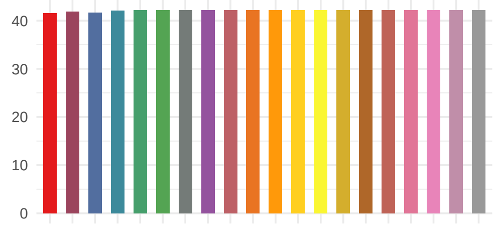
GC content (%)
