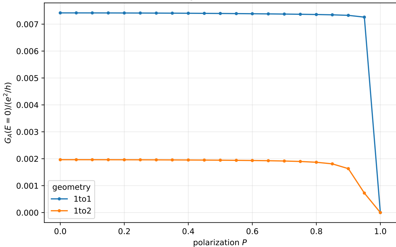
Zero-bias singlet Andreev conductance
